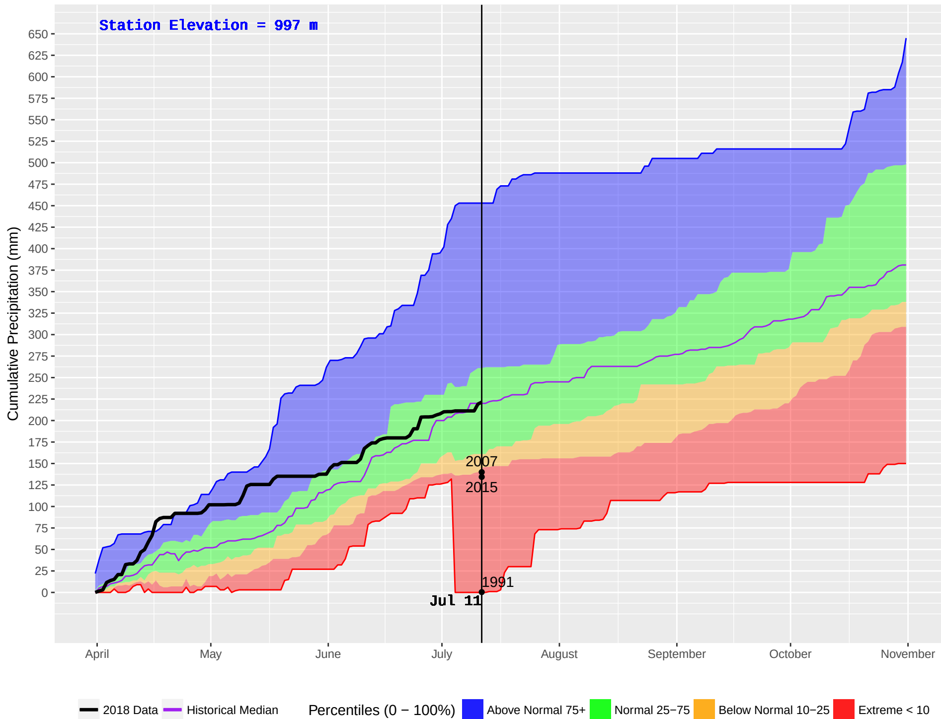
SMALLWOOD (404) : Historical (1991–2016) and Current (2018) Noon Cumulative Precipitation
