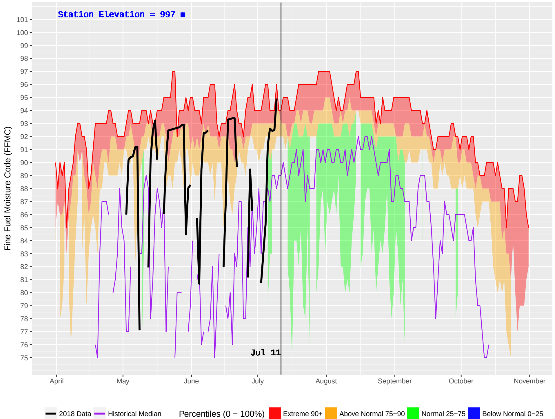
SMALLWOOD (404) : Historical (1991–2016) and Current (2018) Noon Fine Fuel Moisture Code (FFMC)
